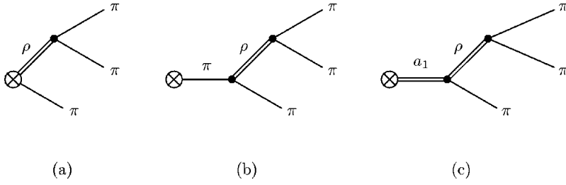
FIG. 2. Resonance-mediated diagrams contributing to the hadronic amplitude T_{\pm\mu}^{(1R)} (a) and (b), and T_{\pm\mu}^{(2R)} (c).
